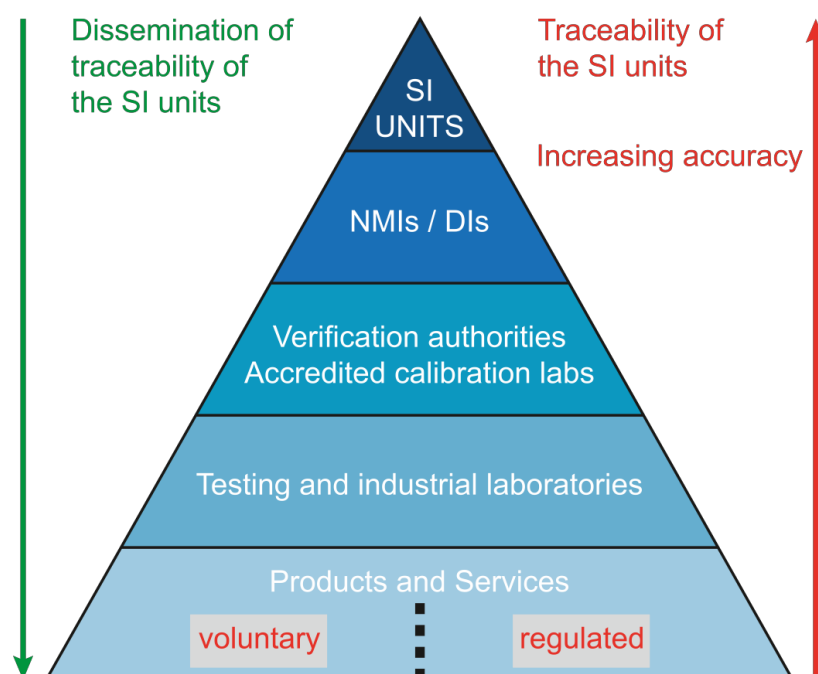
Fig. 7. Traceability pyramid
